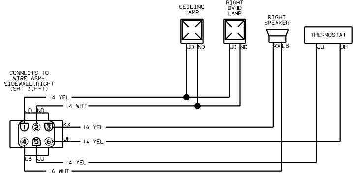
WIRING DIAGRAM-OVHD (WIRE ASM 119701)
