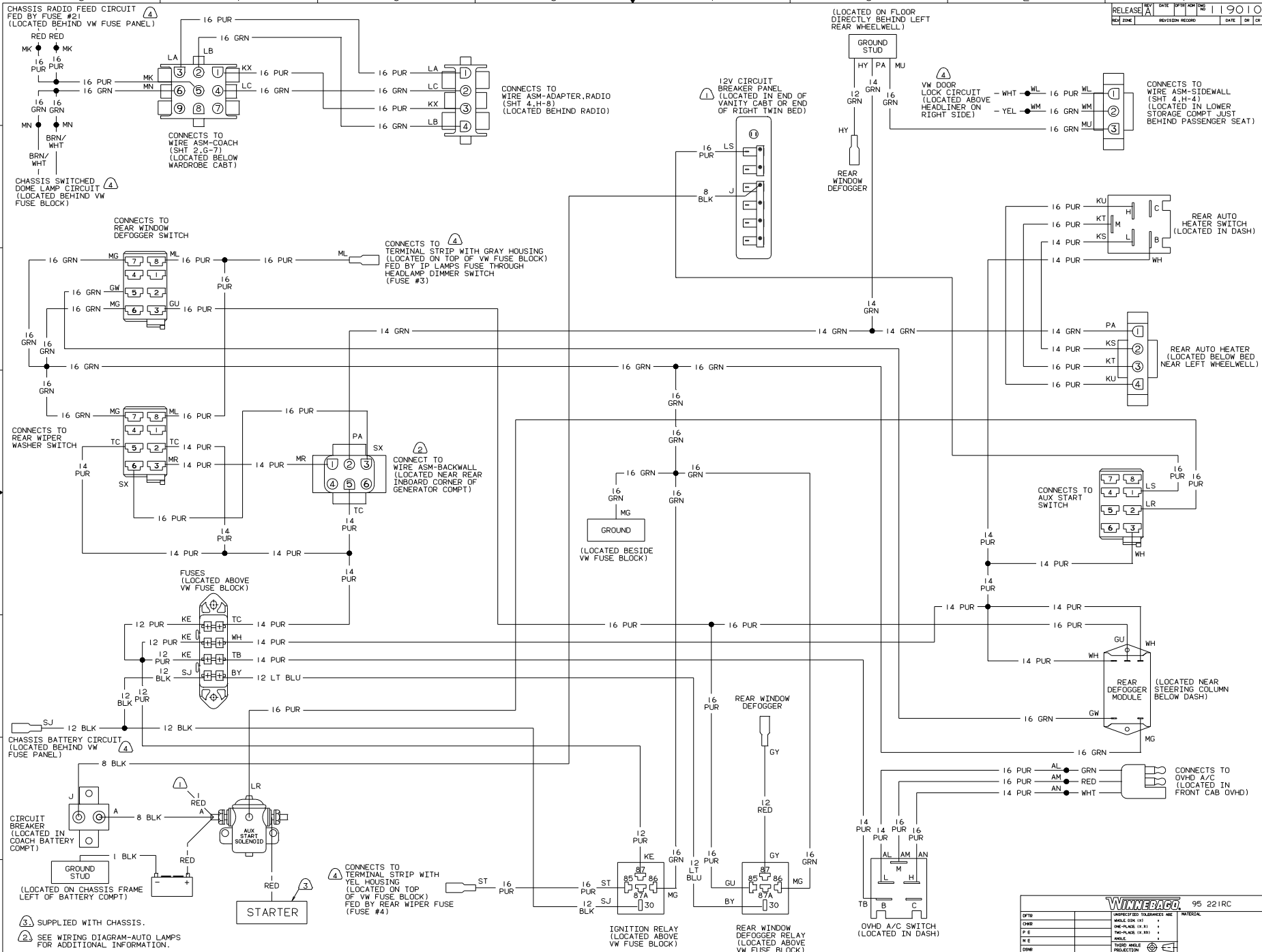
WIRING DIAGRAM-LEFT FRONT (WIRE ASM 119011)
