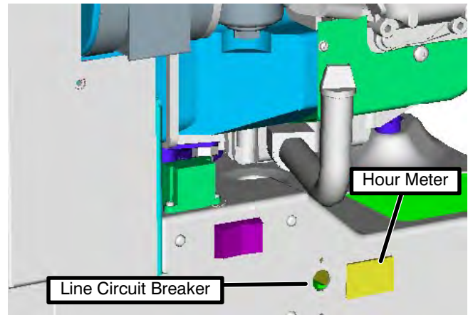
FIGURE 7. LINE CIRCUIT BREAKER
